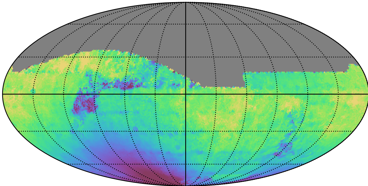
weather_cloudso1v3.4_10yrs All sky z band: Median solarElong
