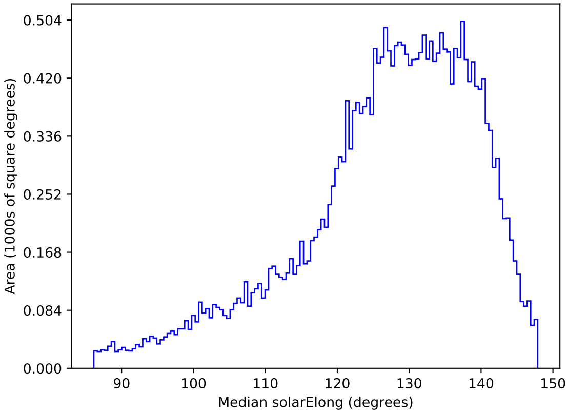
weather_cloudso1v3.4_10yrs All sky z band: Median solarElong
