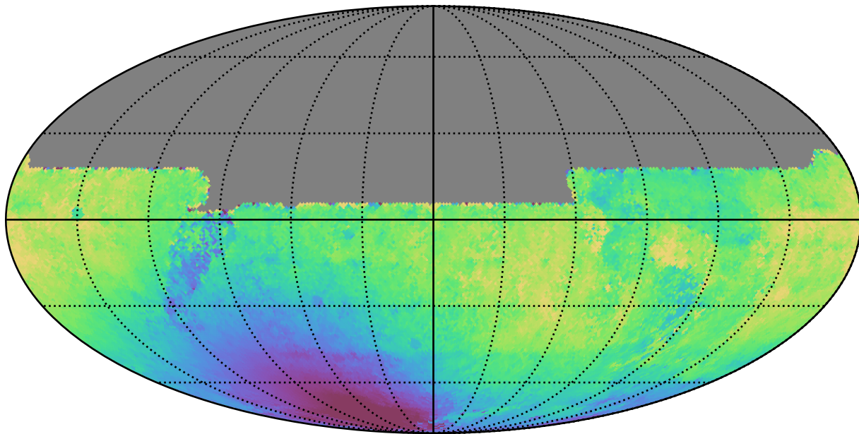
weather_cloudso1v3.4_10yrs All sky y band: Median solarElong
