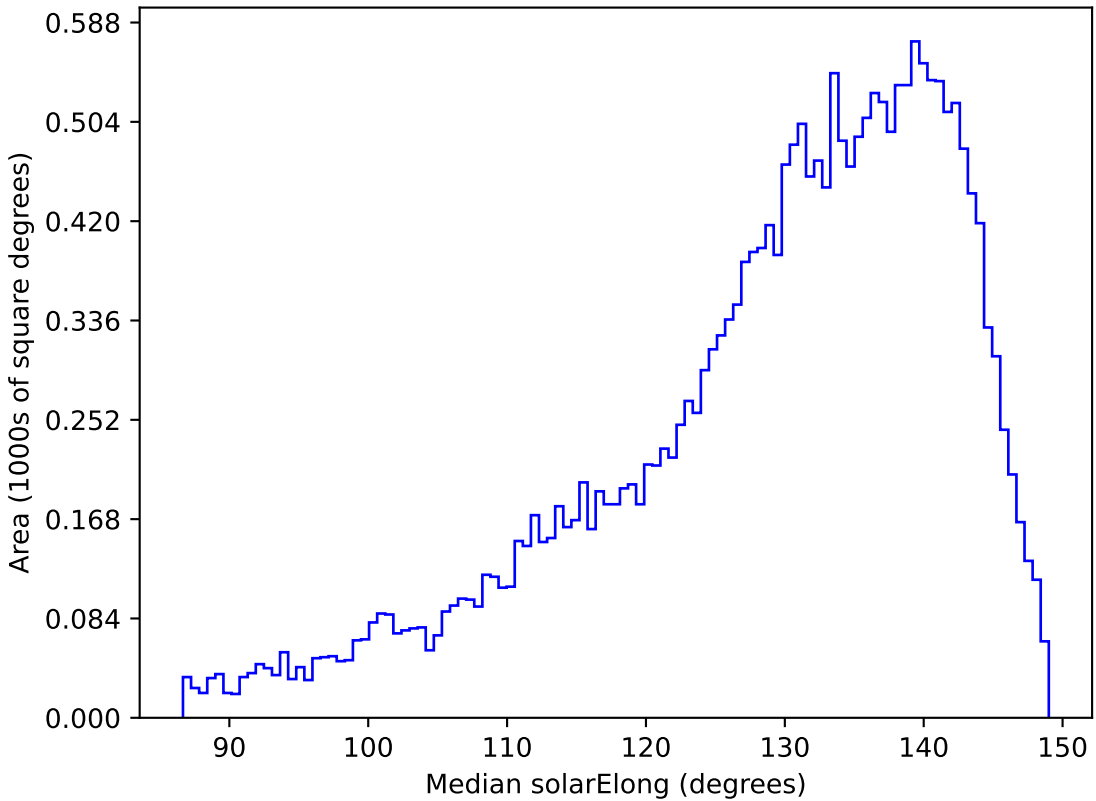
weather_cloudso1v3.4_10yrs All sky y band: Median solarElong
