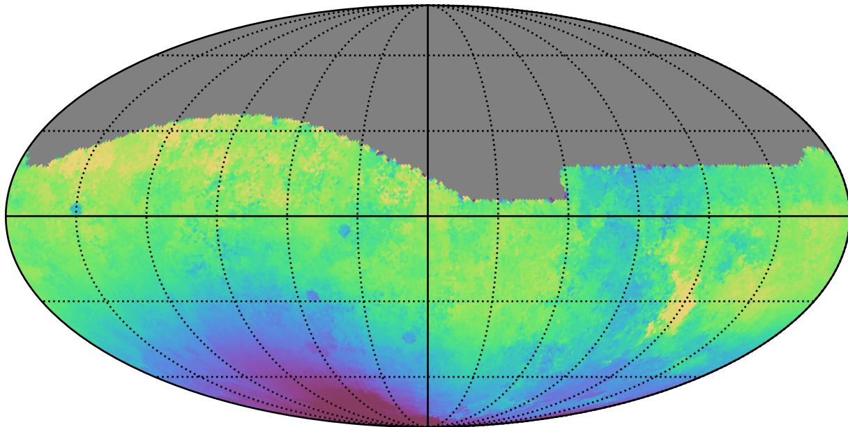
weather_cloudso1v3.4_10yrs All sky g band: Median solarElong
