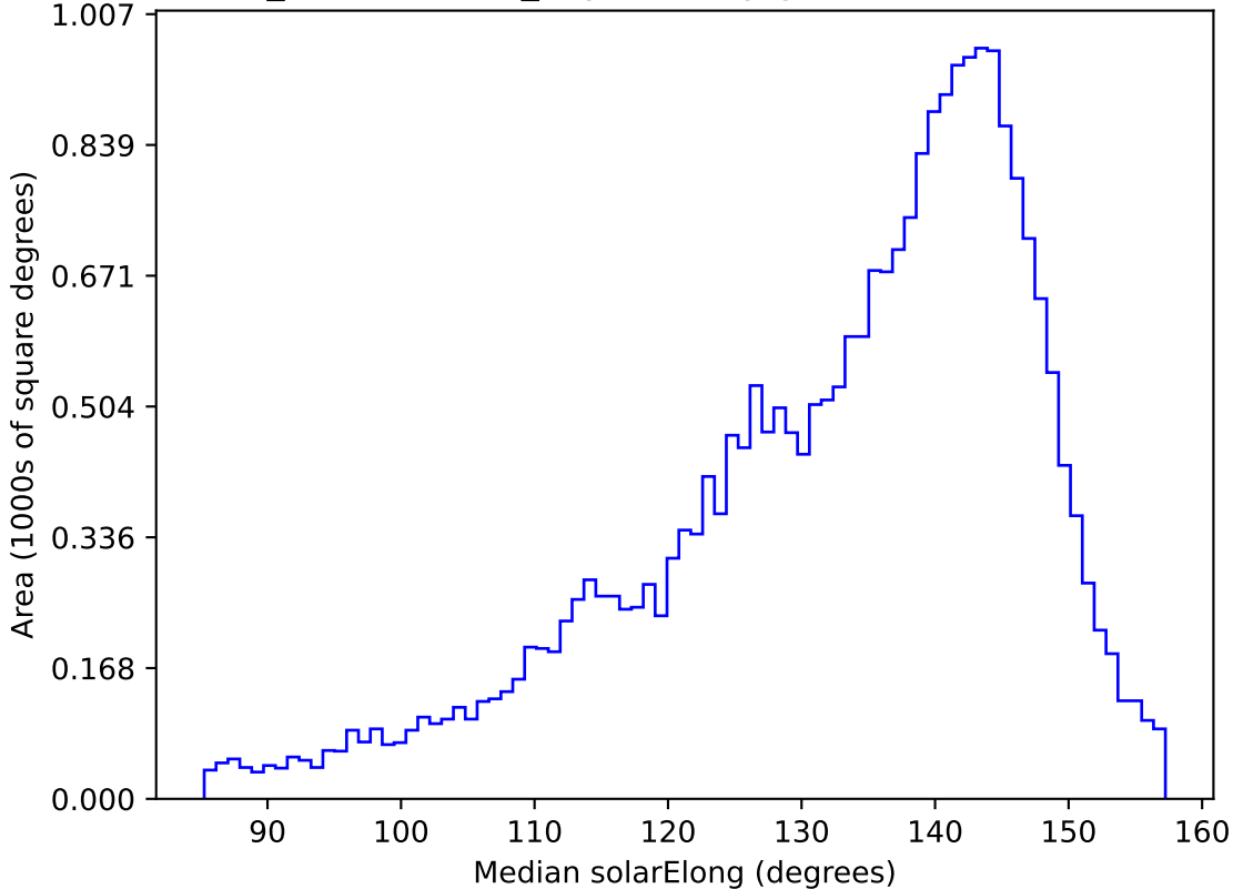
weather_cloudso1v3.4_10yrs All sky g band: Median solarElong
