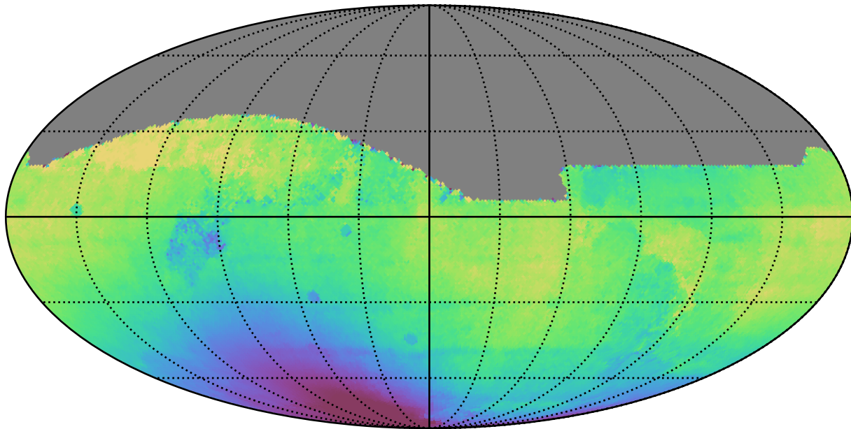
weather_cloudso1v3.4_10yrs All sky all bands: Median solarElong
