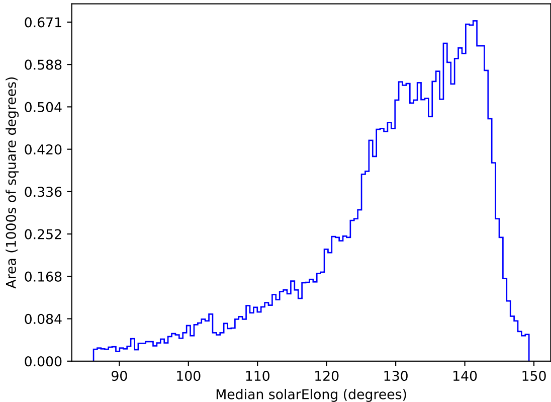
weather_cloudso1v3.4_10yrs All sky all bands: Median solarElong
