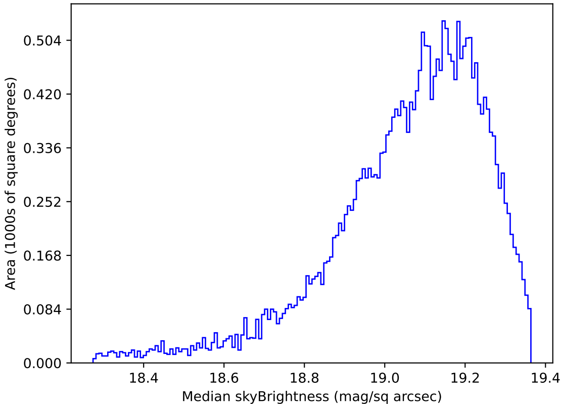
weather_cloudso1v3.4_10yrs Yr 1 z band: Median skyBrightness
