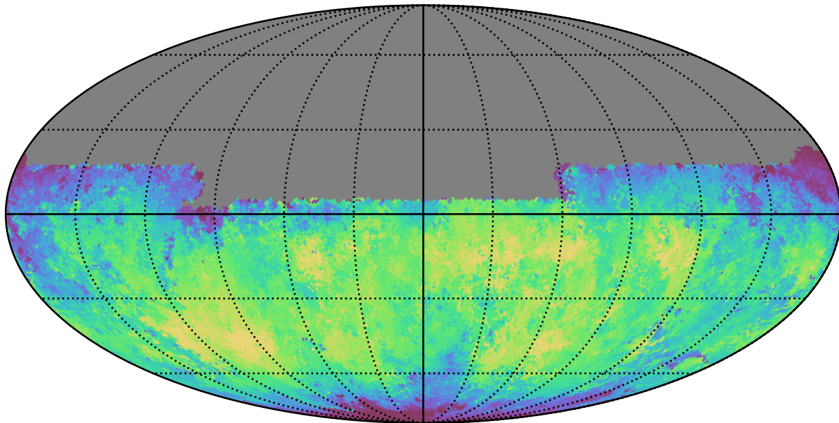
weather_cloudso1v3.4_10yrs Yr 1 y band: Median skyBrightness
