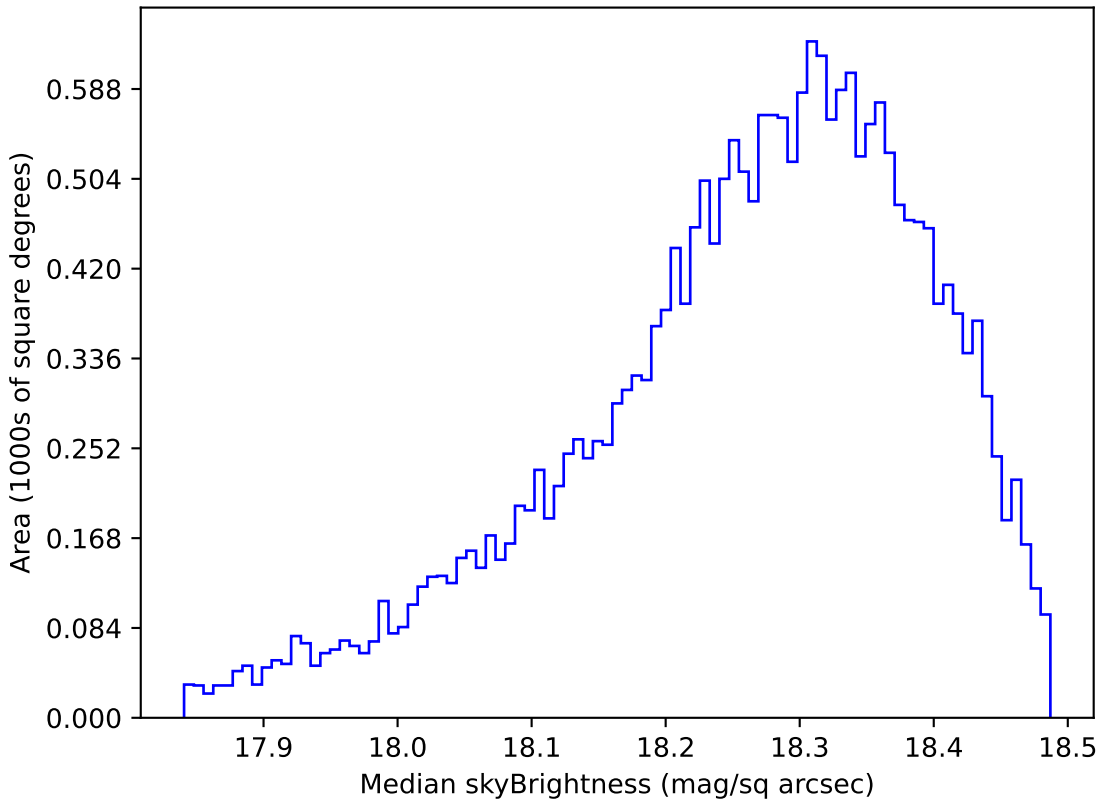
weather_cloudso1v3.4_10yrs Yr 1 y band: Median skyBrightness
