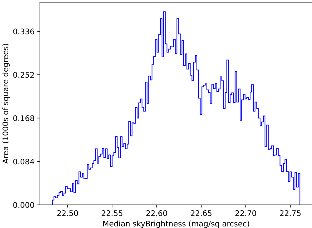
weather_cloudso1v3.4_10yrs Yr 1 u band: Median skyBrightness
