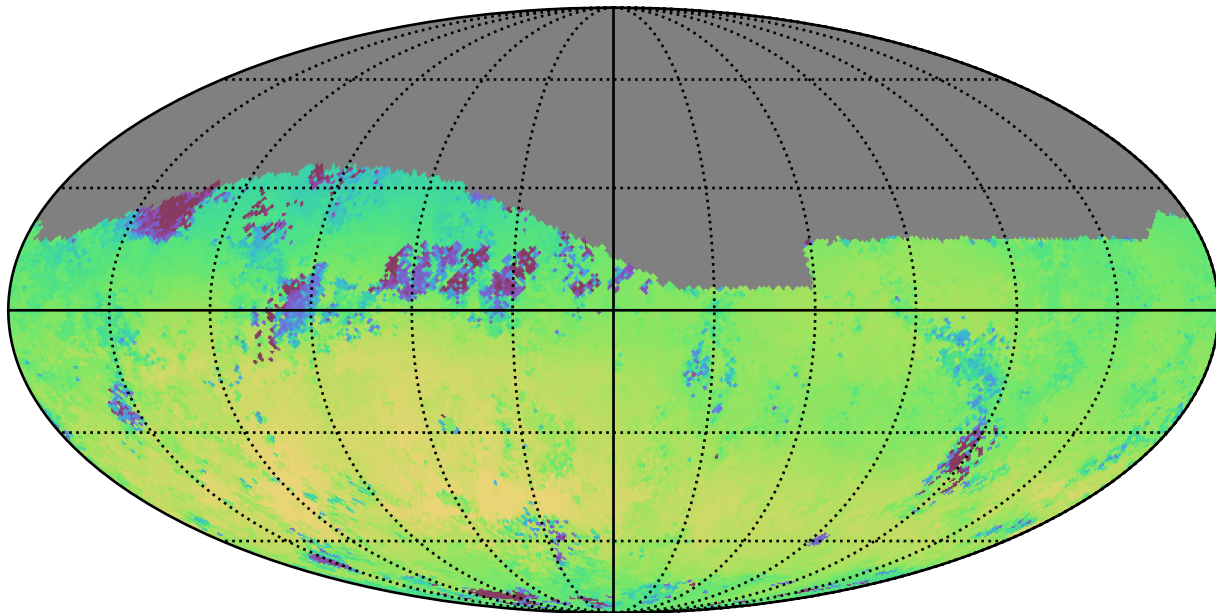
weather_cloudso1v3.4_10yrs Yr 1 r band: Median skyBrightness
