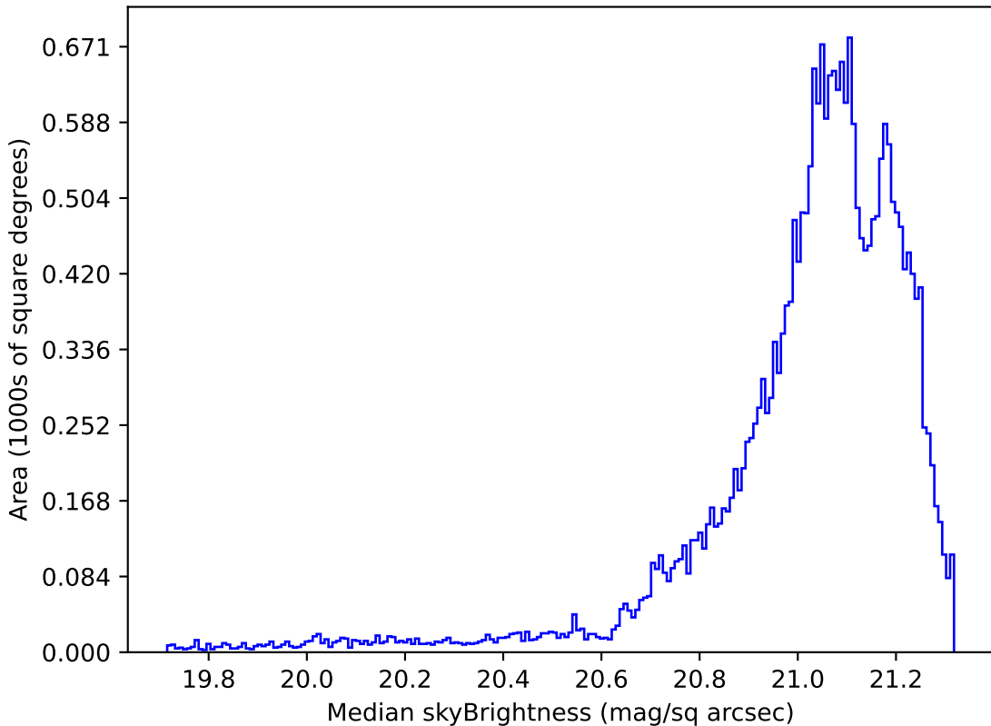
weather_cloudso1v3.4_10yrs Yr 1 r band: Median skyBrightness
