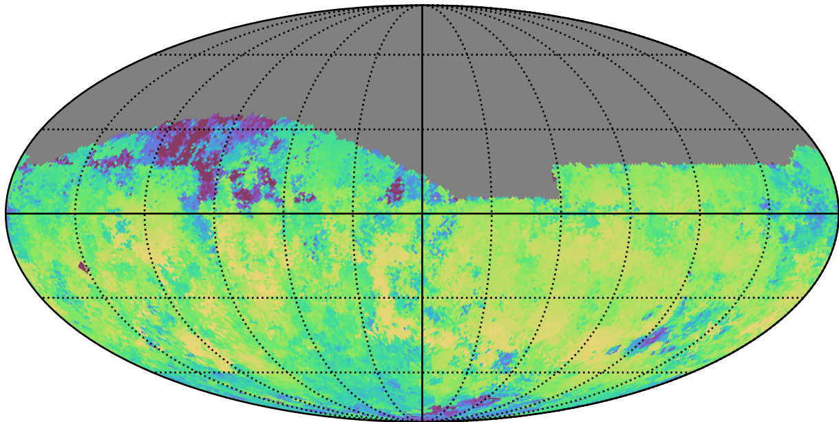
weather_cloudso1v3.4_10yrs Yr 1 i band: Median skyBrightness
