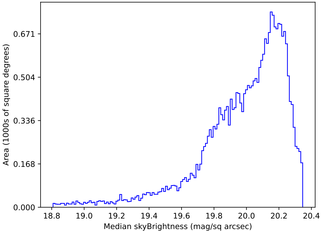
weather_cloudso1v3.4_10yrs Yr 1 i band: Median skyBrightness
