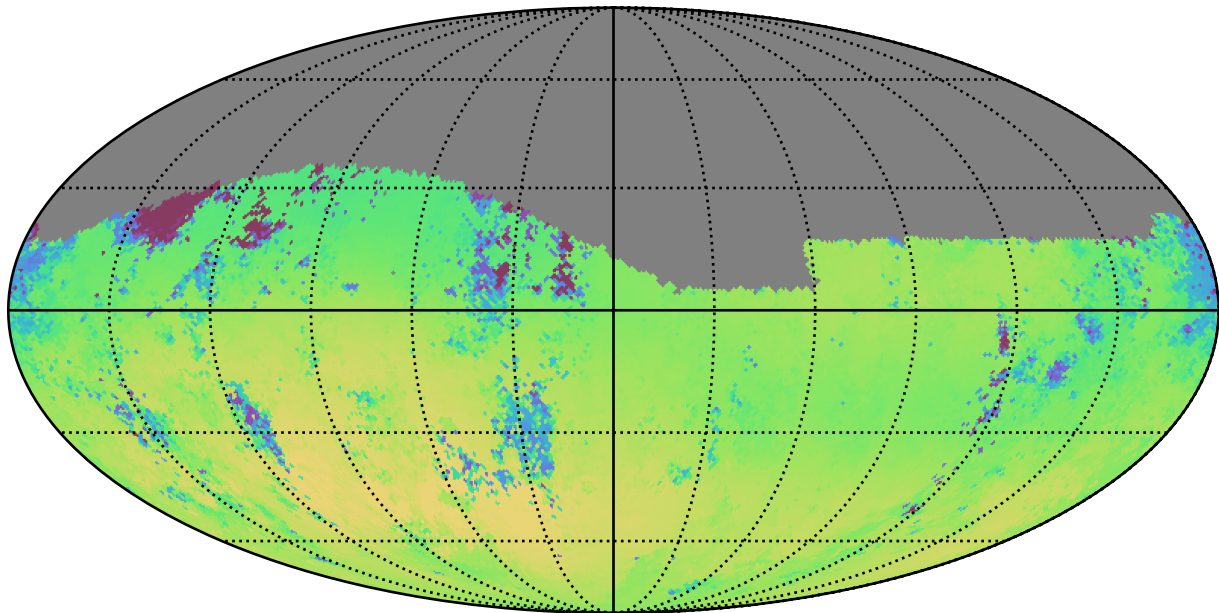
weather_cloudso1v3.4_10yrs Yr 1 g band: Median skyBrightness
