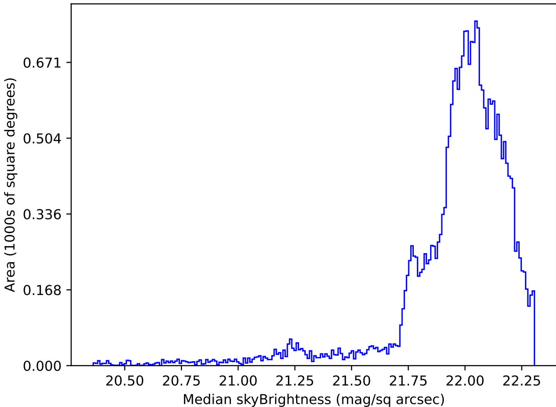
weather_cloudso1v3.4_10yrs Yr 1 g band: Median skyBrightness
