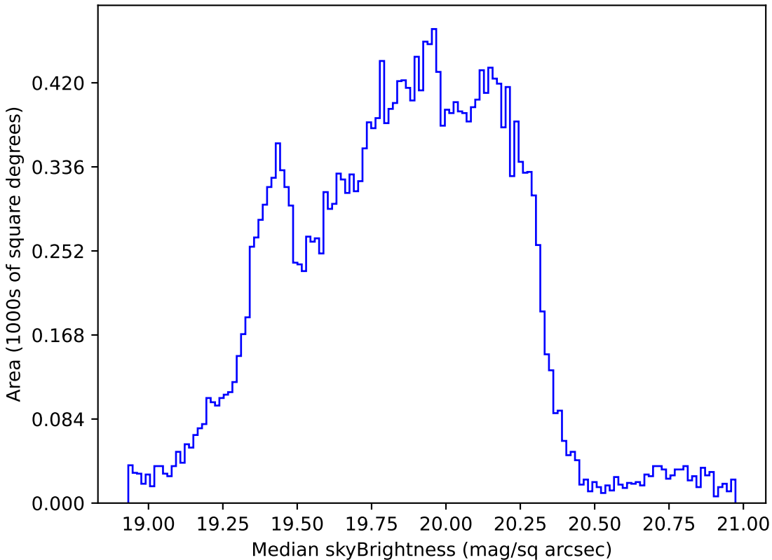
weather_cloudso1v3.4_10yrs Yr 1 all bands: Median skyBrightness
