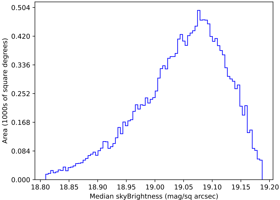
weather_cloudso1v3.4_10yrs WFD z band: Median skyBrightness
