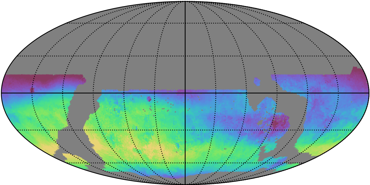
weather_cloudso1v3.4_10yrs WFD u band: Median skyBrightness
