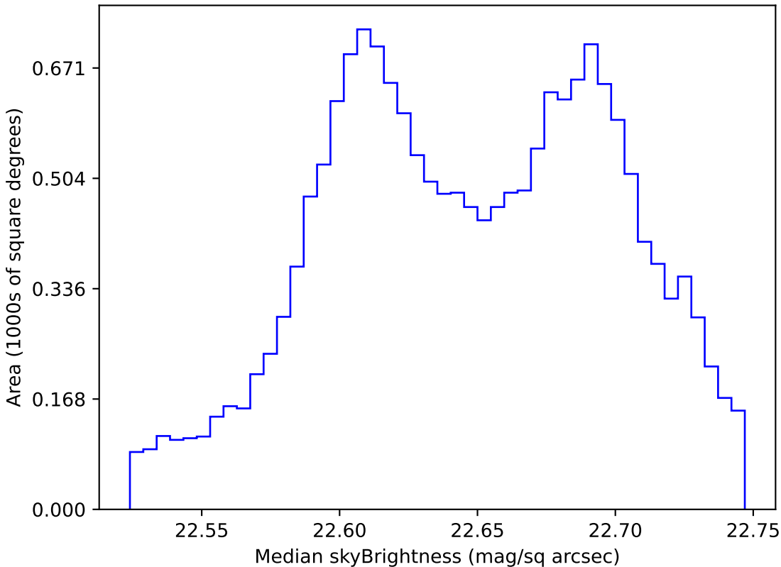
weather_cloudso1v3.4_10yrs WFD u band: Median skyBrightness
