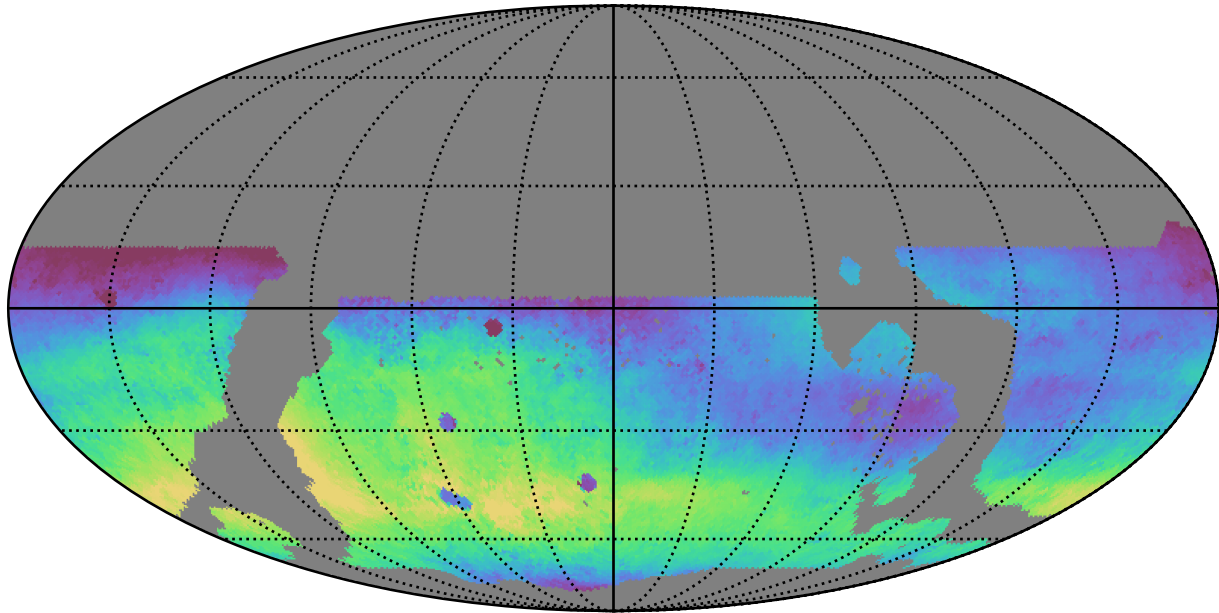
weather_cloudso1v3.4_10yrs WFD r band: Median skyBrightness
