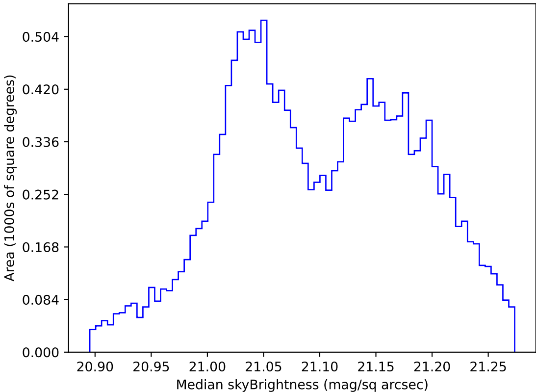
weather_cloudso1v3.4_10yrs WFD r band: Median skyBrightness
