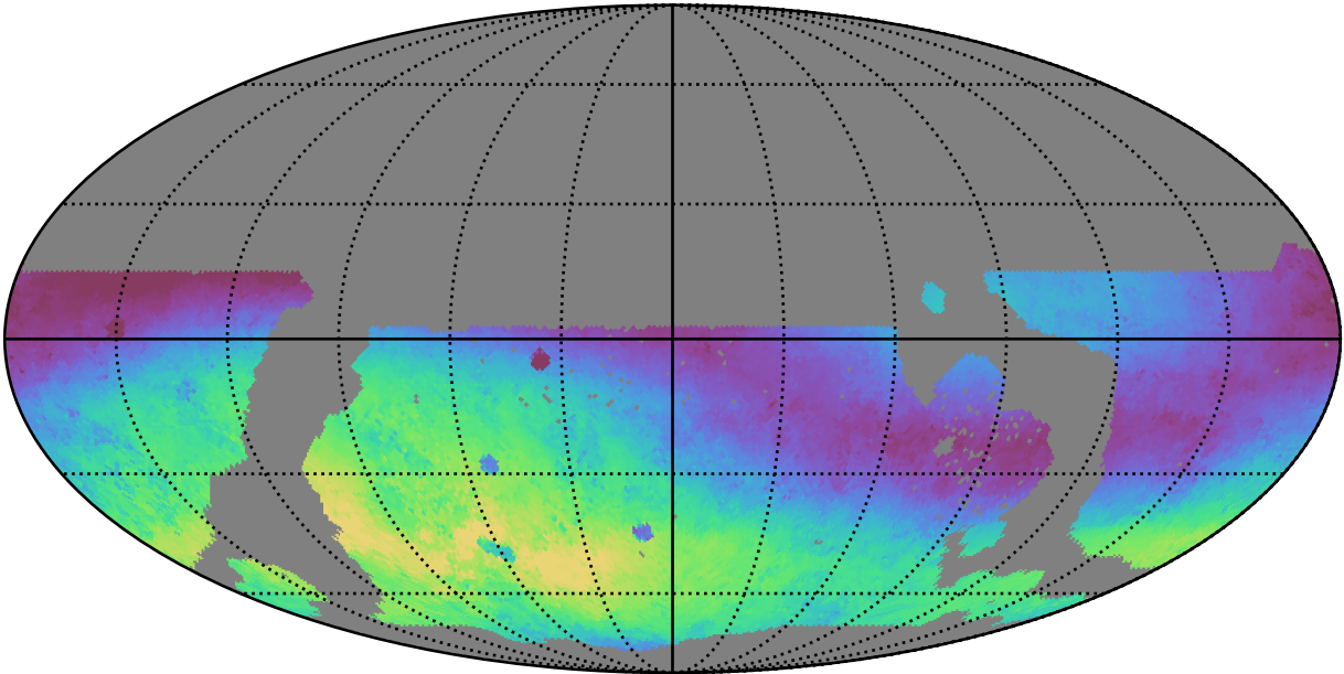
weather_cloudso1v3.4_10yrs WFD g band: Median skyBrightness
