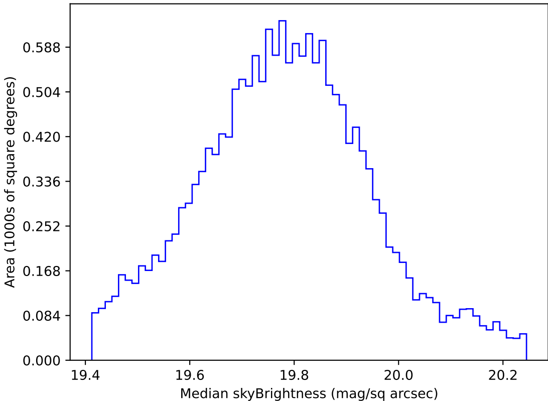
weather_cloudso1v3.4_10yrs WFD all bands: Median skyBrightness
