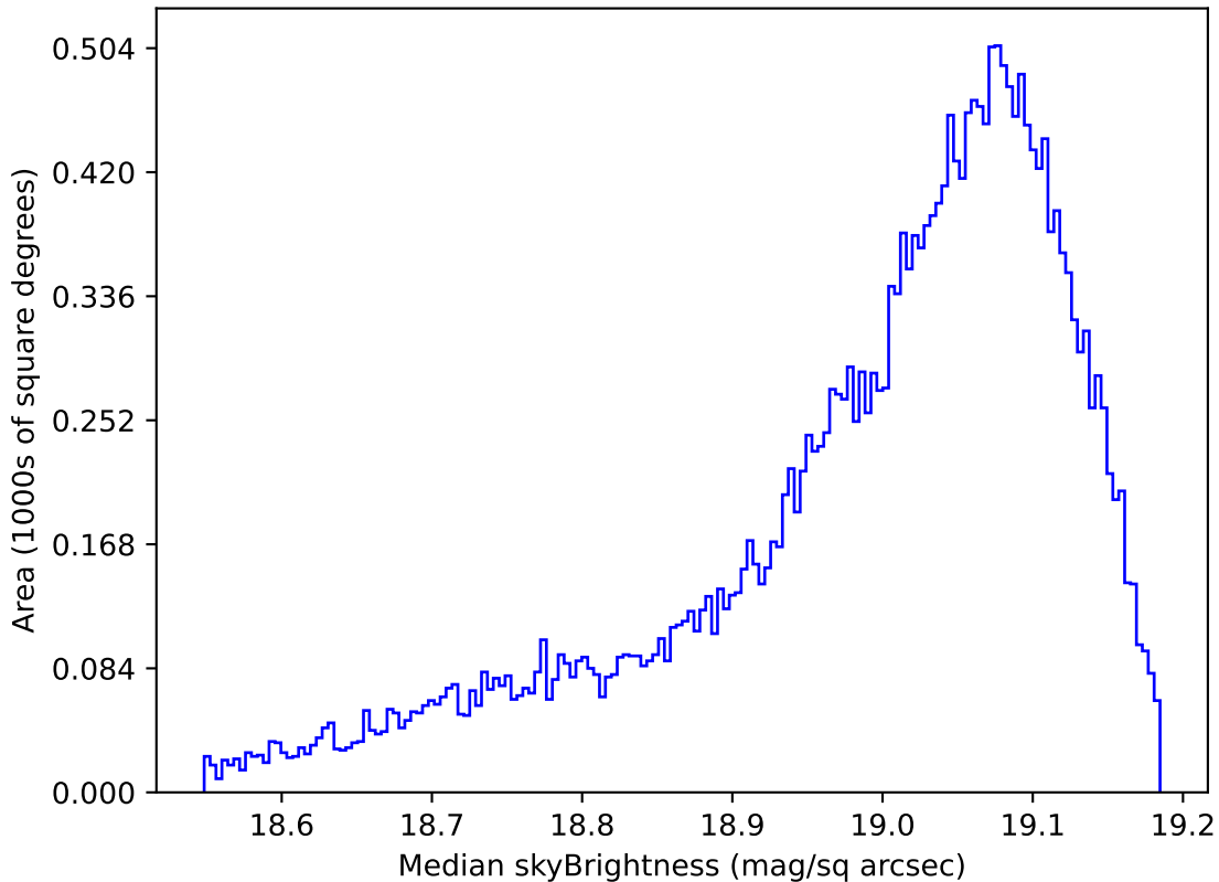
weather_cloudso1v3.4_10yrs All sky z band: Median skyBrightness
