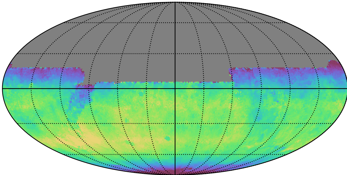
weather_cloudso1v3.4_10yrs All sky y band: Median skyBrightness
