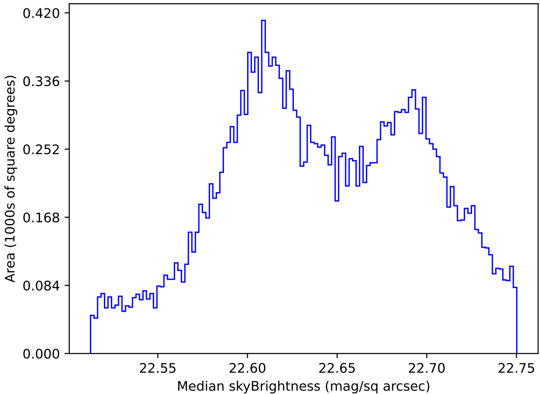
weather_cloudso1v3.4_10yrs All sky u band: Median skyBrightness
