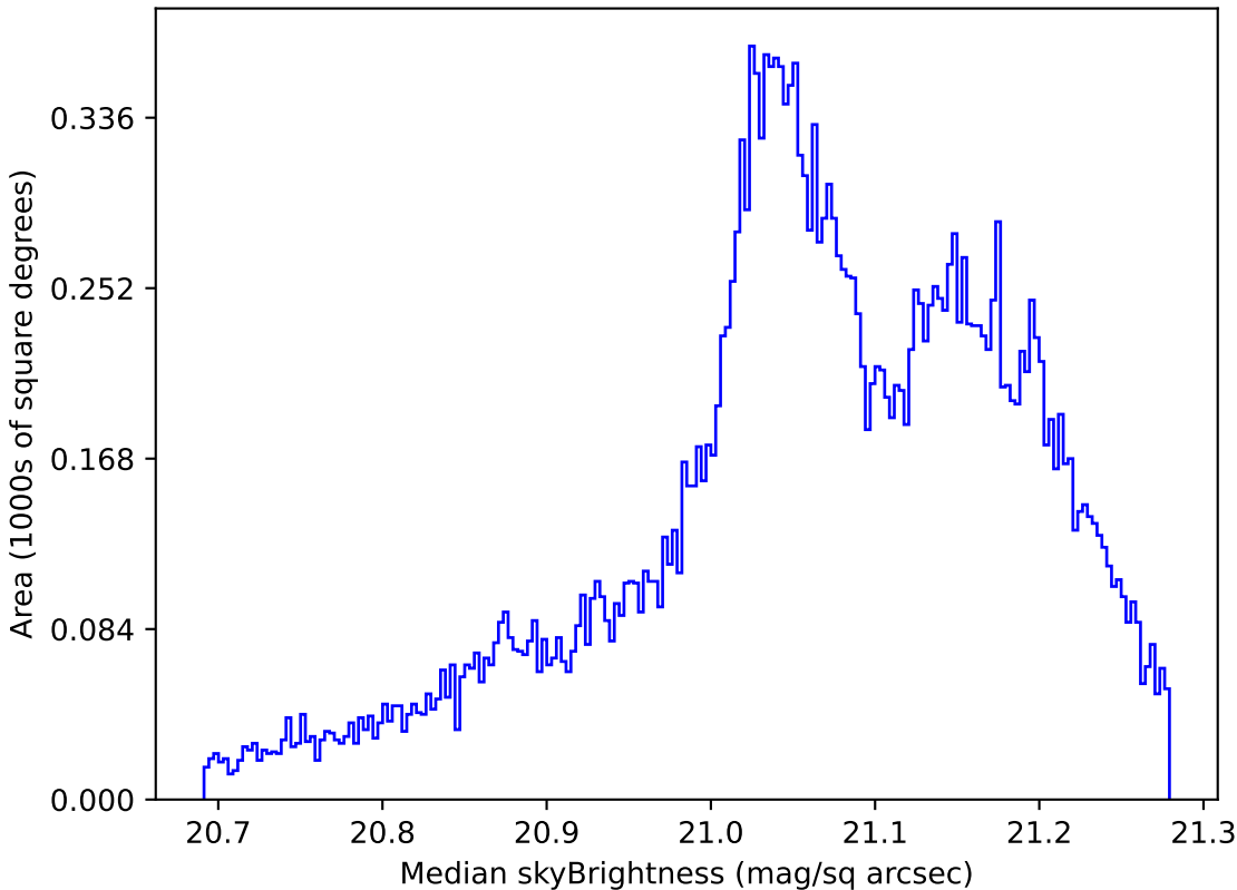
weather_cloudso1v3.4_10yrs All sky r band: Median skyBrightness
