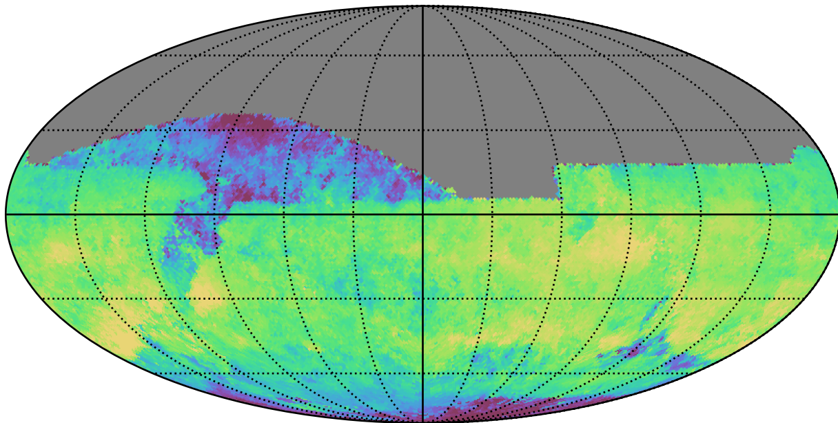
weather_cloudso1v3.4_10yrs All sky i band: Median skyBrightness
