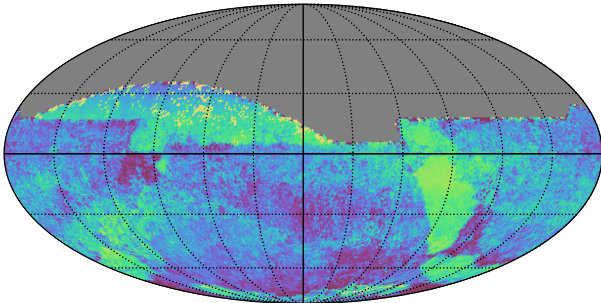
weather_cloudso1v3.4_10yrs All sky all bands: Median skyBrightness
