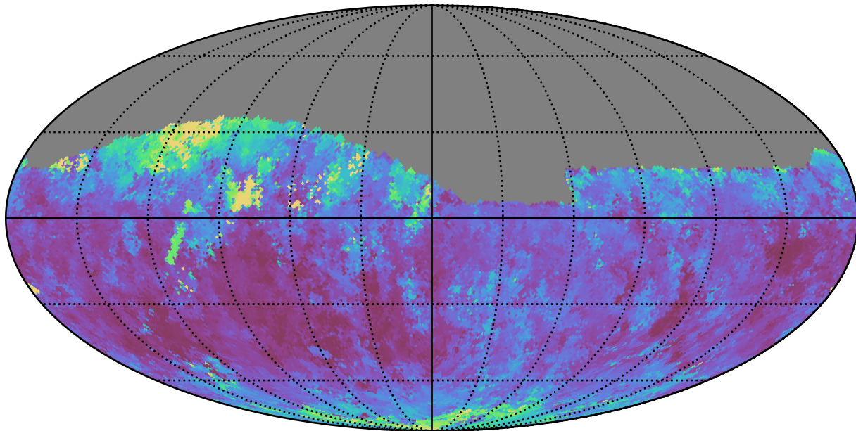
weather_cloudso1v3.4_10yrs Yr 1 z band: Median seeingGeom
