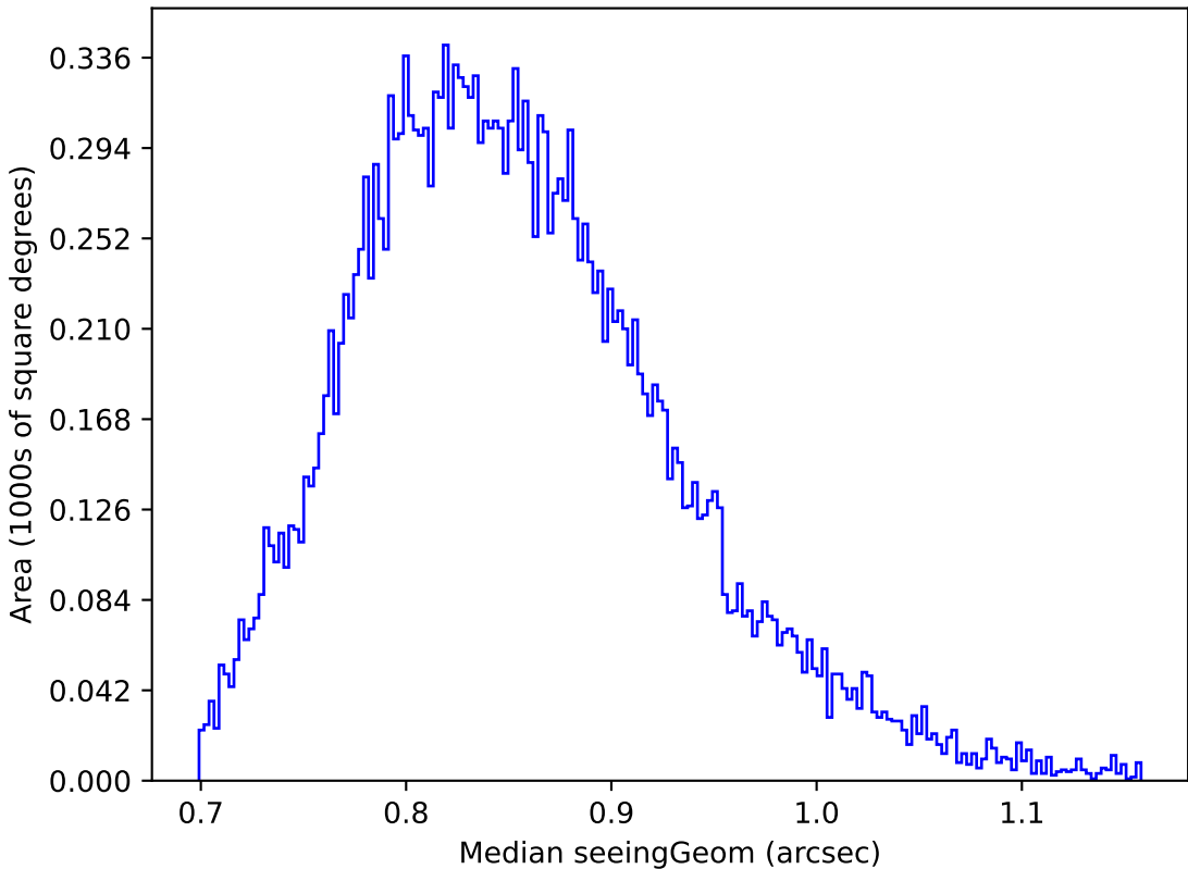
weather_cloudso1v3.4_10yrs Yr 1 y band: Median seeingGeom
