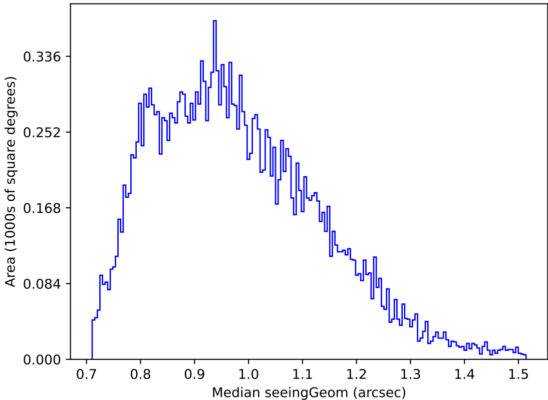
weather_cloudso1v3.4_10yrs Yr 1 u band: Median seeingGeom
