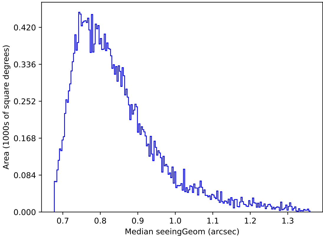
weather_cloudso1v3.4_10yrs Yr 1 i band: Median seeingGeom
