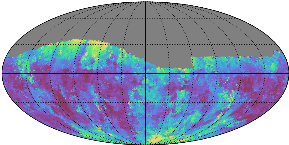
weather_cloudso1v3.4_10yrs Yr 1 g band: Median seeingGeom
