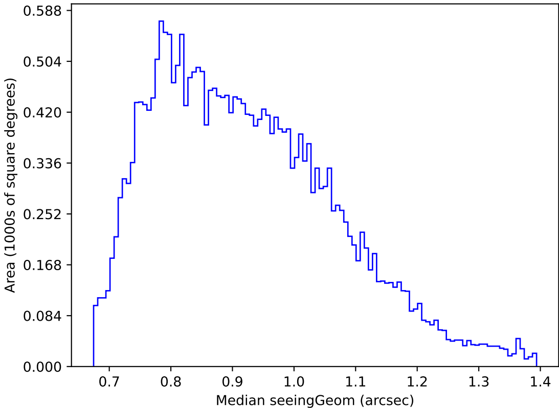
weather_cloudso1v3.4_10yrs Yr 1 g band: Median seeingGeom
