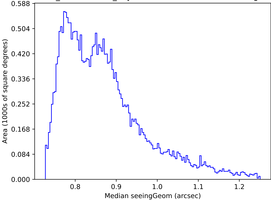
weather_cloudso1v3.4_10yrs Yr 1 all bands: Median seeingGeom
