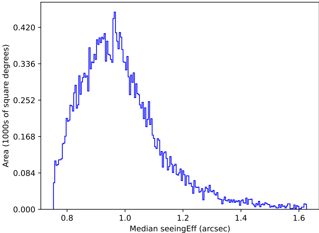
weather_cloudso1v3.4_10yrs Yr 1 z band: Median seeingEff
