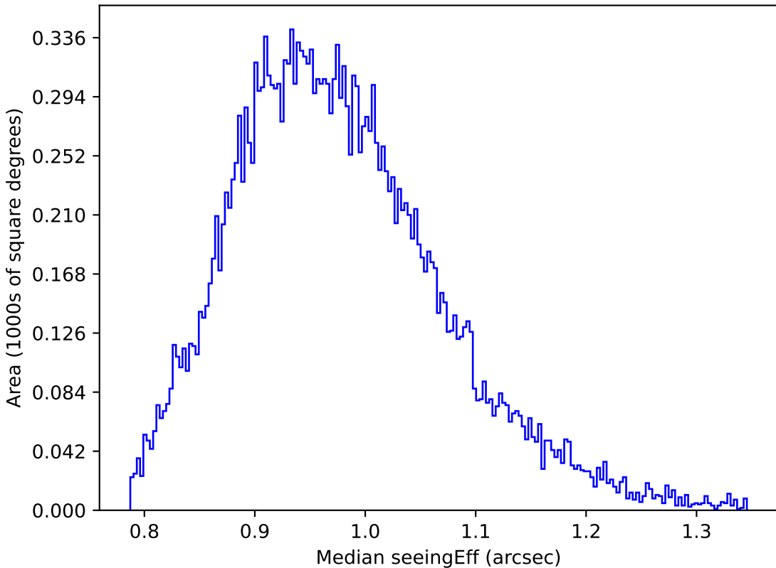
weather_cloudso1v3.4_10yrs Yr 1 y band: Median seeingEff
