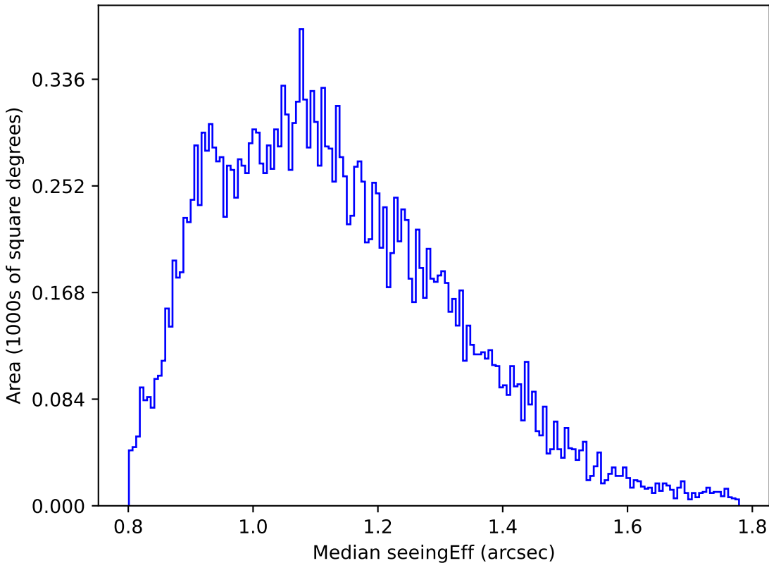
weather_cloudso1v3.4_10yrs Yr 1 u band: Median seeingEff
