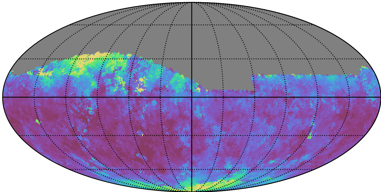
weather_cloudso1v3.4_10yrs Yr 1 i band: Median seeingEff
