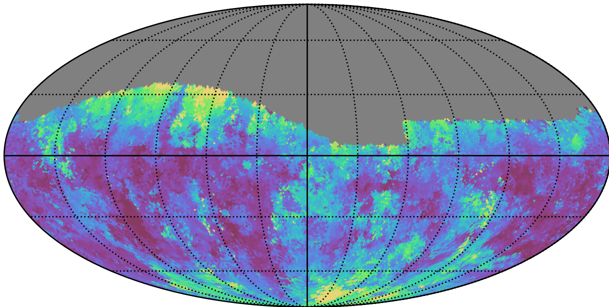
weather_cloudso1v3.4_10yrs Yr 1 g band: Median seeingEff
