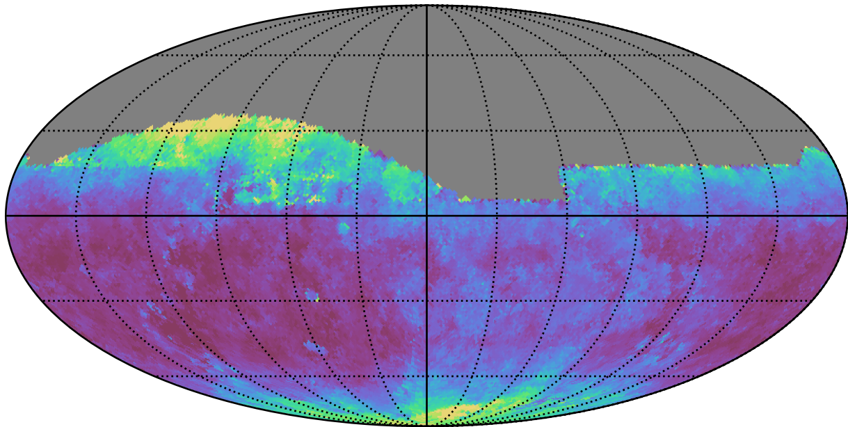
weather_cloudso1v3.4_10yrs Yr 1 all bands: Median seeingEff
