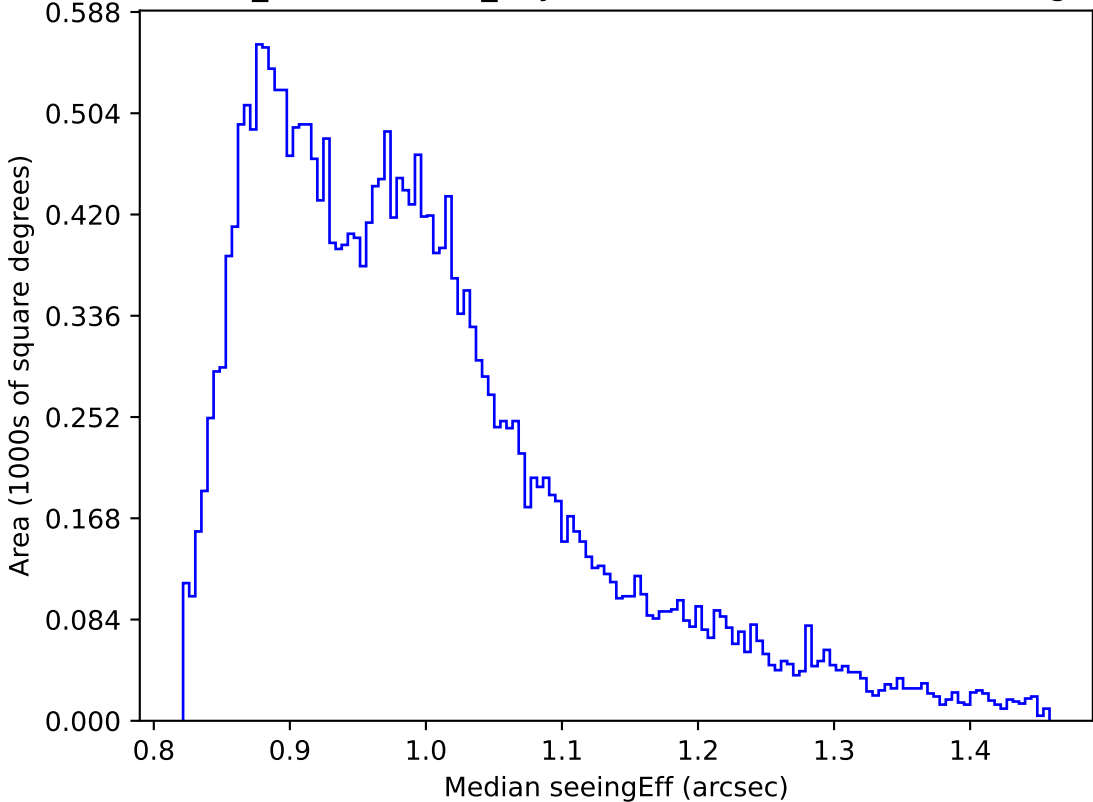
weather_cloudso1v3.4_10yrs Yr 1 all bands: Median seeingEff
