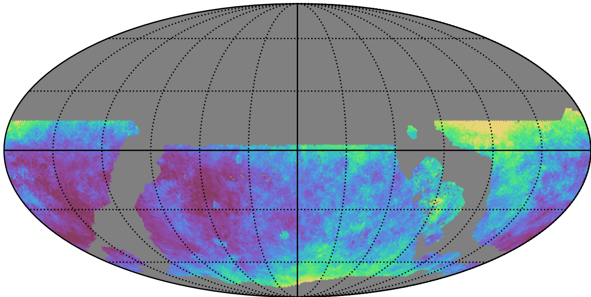
weather_cloudso1v3.4_10yrs WFD y band: Median seeingEff
