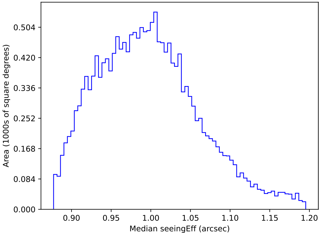
weather_cloudso1v3.4_10yrs WFD y band: Median seeingEff
