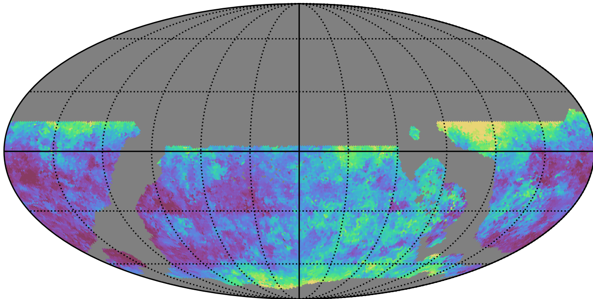
weather_cloudso1v3.4_10yrs WFD u band: Median seeingEff
