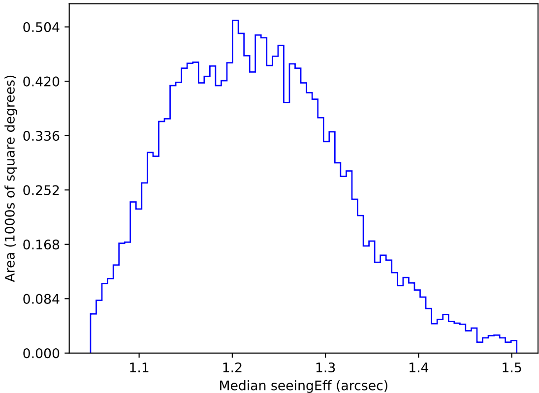
weather_cloudso1v3.4_10yrs WFD u band: Median seeingEff
